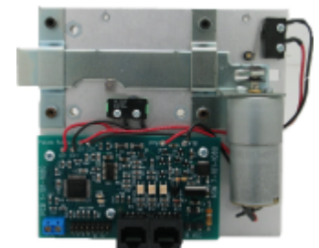
E-locX Internal
